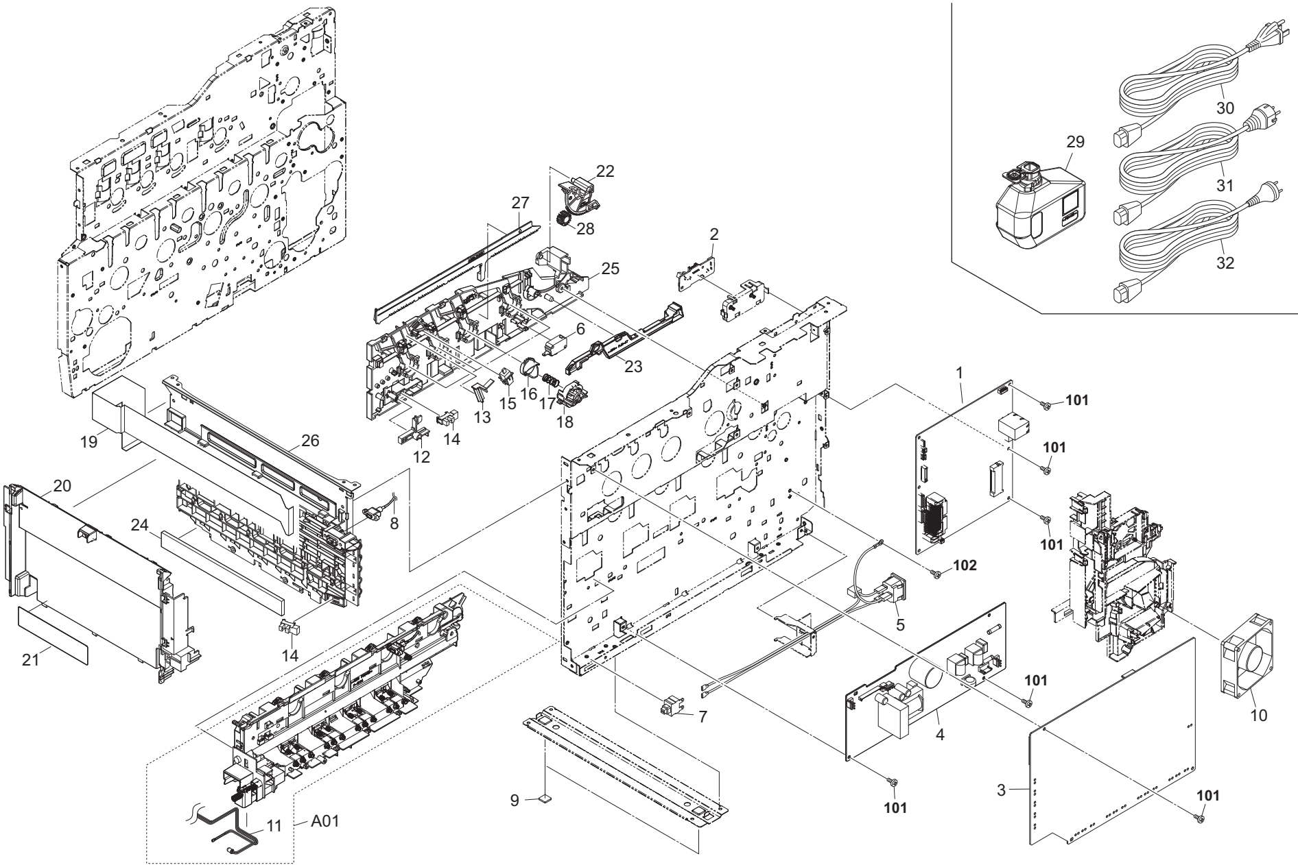
FIG. 13 Electrical Components 2
